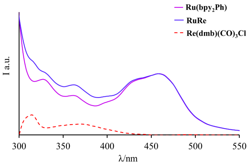
Figure 5.4. Excitation spectra of Ru(bpy 2 Ph) (violet solid line) and RuRe (blue solid line) at 610 nm and difference spectrum (red dashed line).
