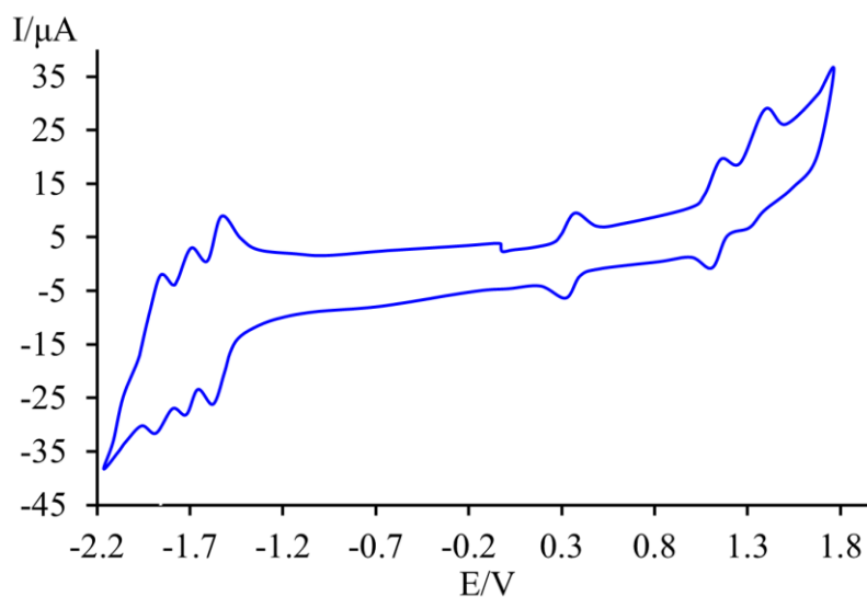
Figure 5.18. Cyclic voltammogram of Ru 2 Re (0.5 mM) in argon purged MeCN at room temperature using \text{Bu}_4\text{NPF}_6 (0.05 M) as supporting electrolyte. As internal reference, it was used the redox couple ferrocene/ferrocenium (395 mV vs. SCE in acetonitrile). Scan rate 200 mV/s.
