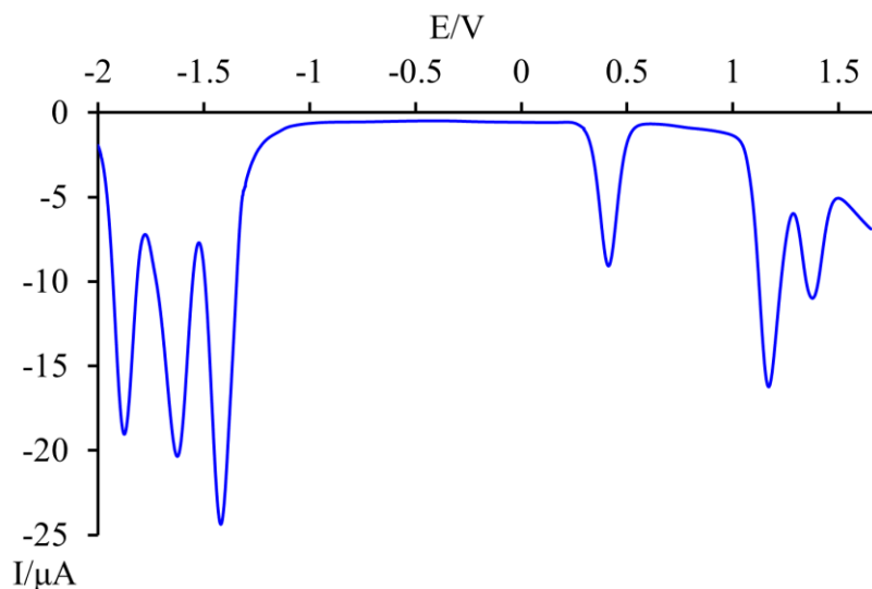
Figure 5.17. DPV analysis of Ru 2 Re (0.5 mM) in argon purged MeCN at room temperature using \text{Bu}_4\text{NPF}_6 (0.05 M) as supporting electrolyte. As internal reference, it was used the redox couple ferrocene/ferrocenium (395 mV vs. SCE in acetonitrile). Scan rate 20 mV/s.
