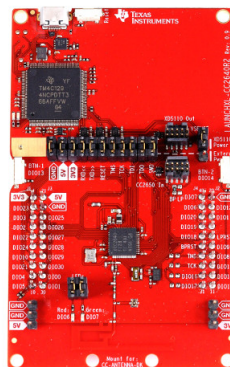
Figure 3.5: CC2640R2F LaunchPad
