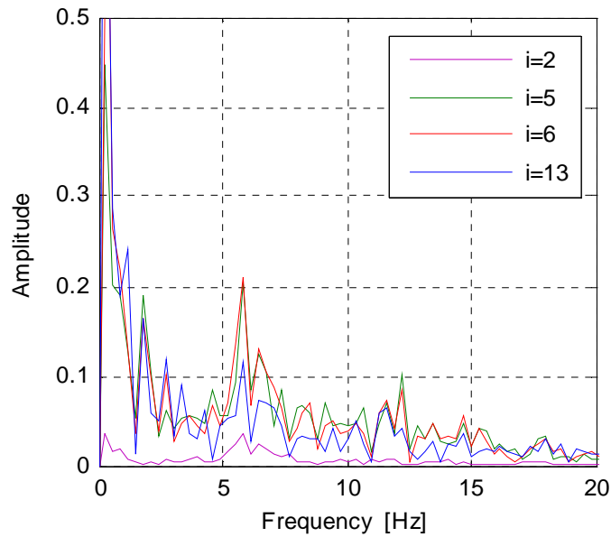
Fig.5.16: Frequency spectrum for J1 = 0.65 \text{ m/s} - Jg = 2.26 \text{ m/s}
