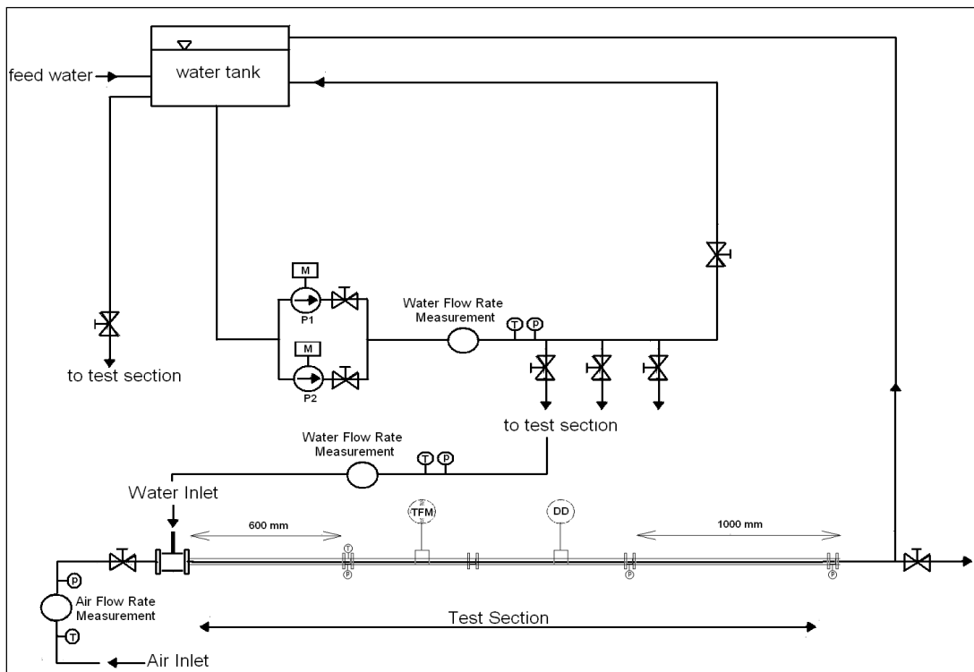
Fig.6.1: Experimental facility
