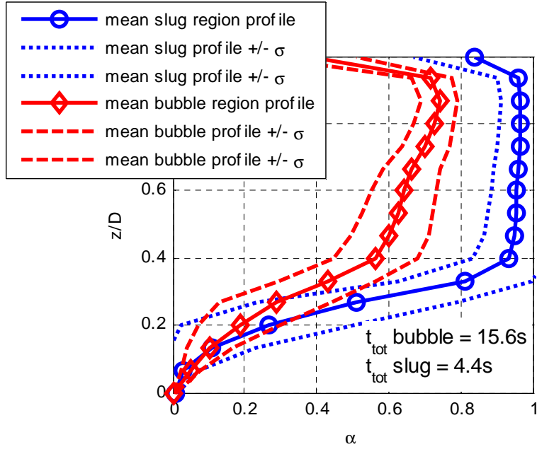
Fig.5.15: Void fraction profile analysis for the “quasi periodic” flows at J1 = 0.65 \text{ m/s} - Jg = 2.26 \text{ m/s}
