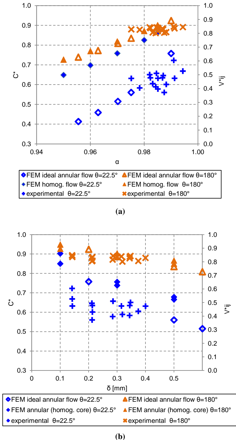
Fig.8.34: Comparison between experimental and numerical external electrodes results at 22.5° and 180° for two-phase flow. Void fraction dependency (a) and film thickness dependency (b)
