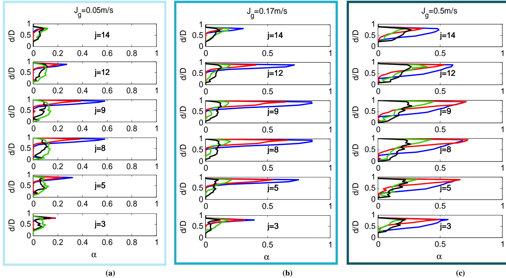
Fig.5. 33: Velocities dependency: Vertical Profiles
