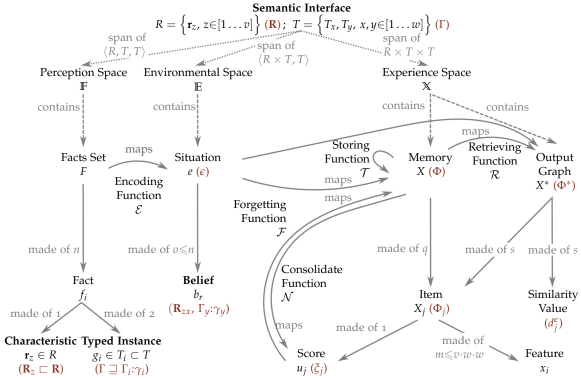
Figure 10.3: A glossary of the symbols (in black), and their relations (in grey), defined in this paper for representing a type of memory based on the SIT algorithm. For a quick reference, we show in red some elements of the ontology that are relevant for implementing the related black symbols, which are motivated during the description of the architecture.
