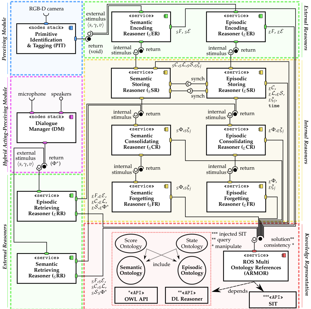
Figure 10.6: The software architecture where we deploy our design patten for managing the semantic and the episodic memory.
