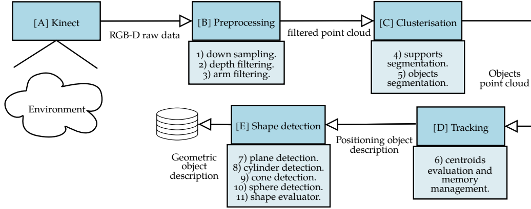
Figure 2.1: Abstract representation of the system’s architecture: components (blue squares) represent information sources and computational units, exchanged data (arrows) are related to the internal information flow.
