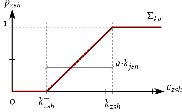
Figure 8.2: A general representation of a minimal fuzzy cardinality restriction based on a right-shoulder membership function \Sigma_{k_a} = \mathcal{C}(k_{zsh}, a) .
