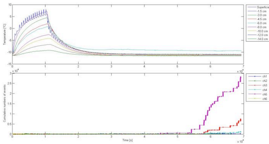
Figure 5.14: Temperature distribution during the first step of the freezing process.
