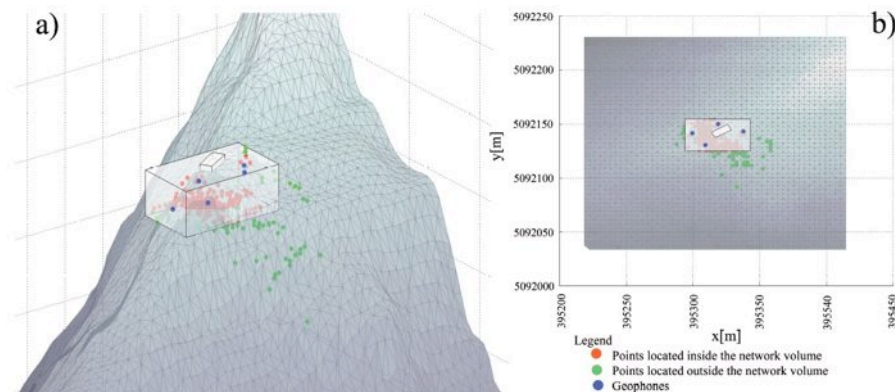
Figure 3.4: Location results of the whole data set (615 events) in relation to the network volume; a) perspective view showing the points inside (in red) and outside (in green) the volume: it is possible to notice that most of the points located inside the network boundaries correspond to the more superficial events; b) projection of the results on the horizontal plane. ([111] Occhiena, 2011).
