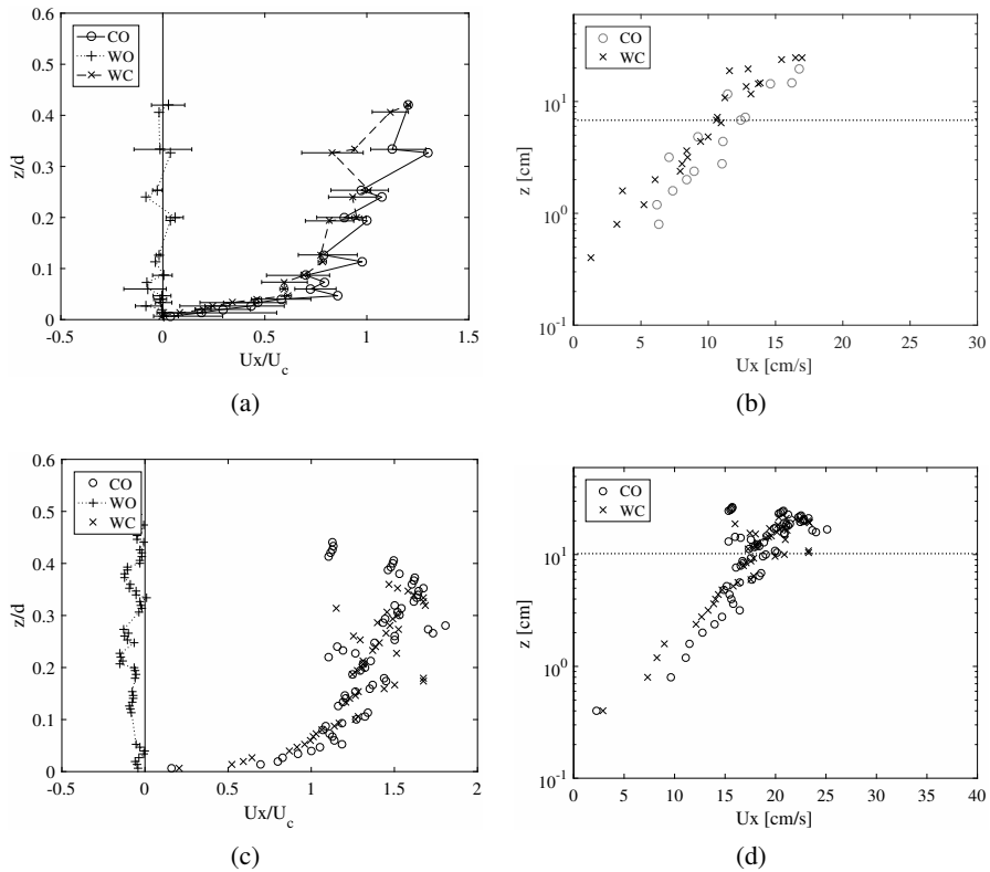
Figure 6.19: Velocity profiles along the x direction in the GB case Run19 (CO), Run26 (WO), Run22 (WC, WD) d=0.6 m, H=0.12 m, T=2 s (a) VS1-VS5, (c) VP1; logarithmic profile of Run19 (CO) and Run22 (WC, WD) (b) VS1-VS5, (d) VP1.
