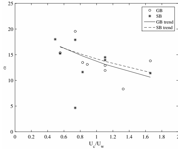
Figure 6.22: Mean flow direction versus the current to wave velocity ratio.
