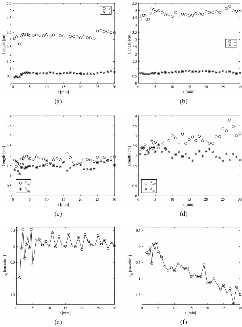
Figure 4.9: Reg 10 test morphodynamic at P_1 (left panel) and P_2 (right panel): (a), (b) Wavelength \lambda and height \eta time evolution; (c), (d) Half-wavelengths \lambda_{on} and \lambda_{off} time evolution, see sketch in Figure 4.1c; (e), (f) Ripple crests migration velocity v_0 time.
