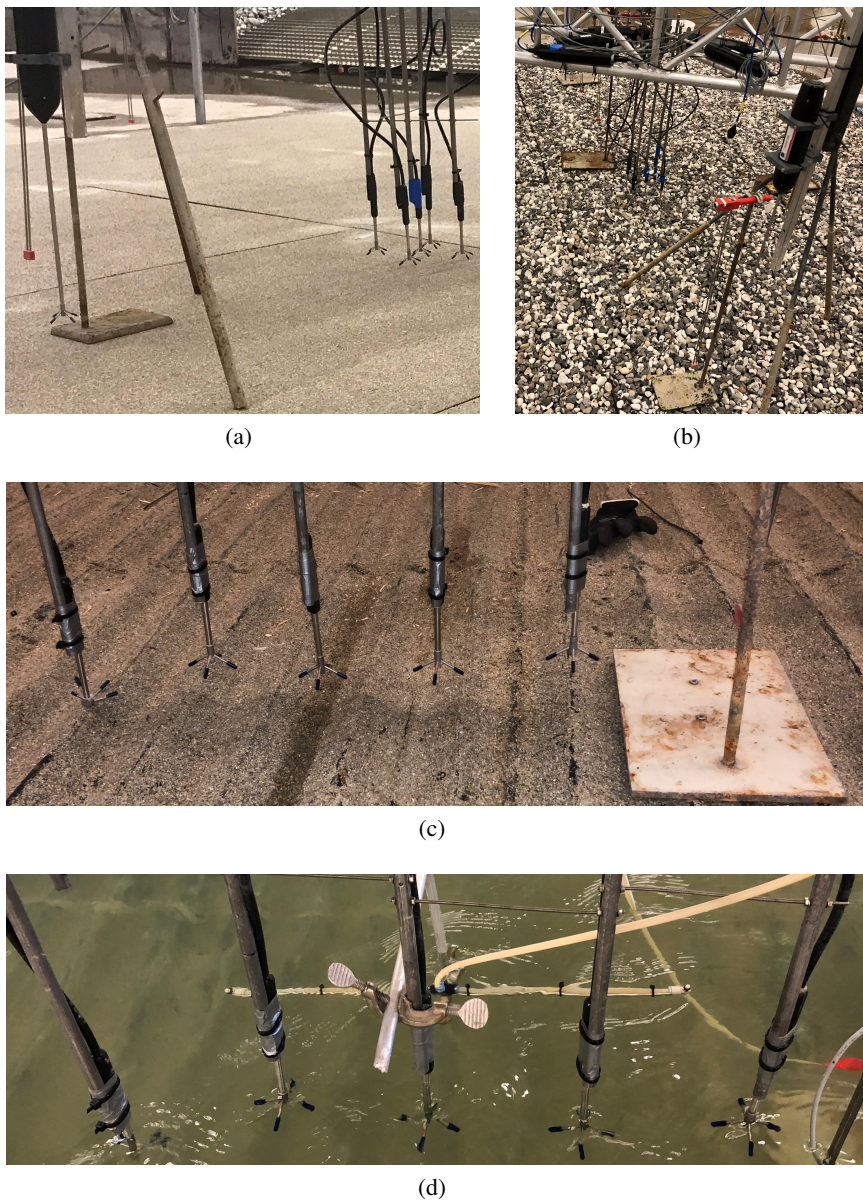
Figure 6.4: Vectrinos positioning: (a) sand bed; (b) gravel bed; (c) rippled bed; (d) seeding system.
