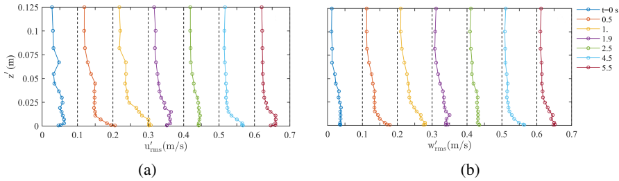
Figure 5.9: Turbulent intensities at x=50.78 \text{ m} . (a) Cross-shore turbulent intensity; (b) Vertical turbulent intensity. The data of each phase are shifted forward by 0.1 \text{ ms}^{-1} compared to those of the previous phase.
