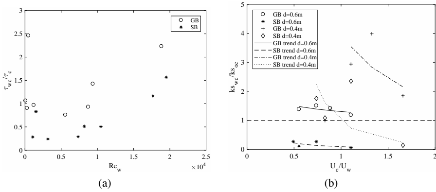
Figure 6.25: (a) Non dimensional wall shear stress as a function of wave Reynolds number; (b) non dimensional equivalent roughness versus the current to wave velocity ratio.
