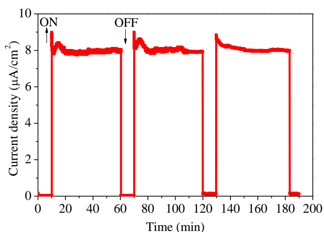
Figure 4.9. Photocurrent stability vs. time of PANI/ \text{TiO}_2 film obtained by chrono-amperometric ( I-t ) technique at an applied potential of 0.26 V vs. Ag/AgCl ( 1.23 V vs. RHE) under illumination with ON/OFF cycles
