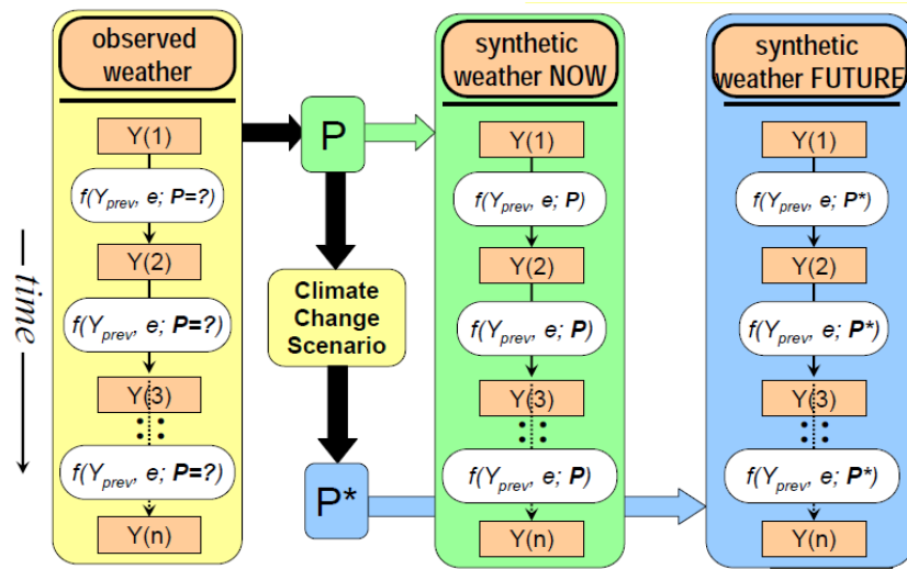
Figure 24. Scheme of using the weather generator Y(t) = weather series; f(.) = underlying model of the weather generator; e = random vector; P = set of WG parameters derived from the observed series; P^* = WG parameters representing future climate and obtained by modifying P according to the climate change scenario (from Dubrovsky 2009).
