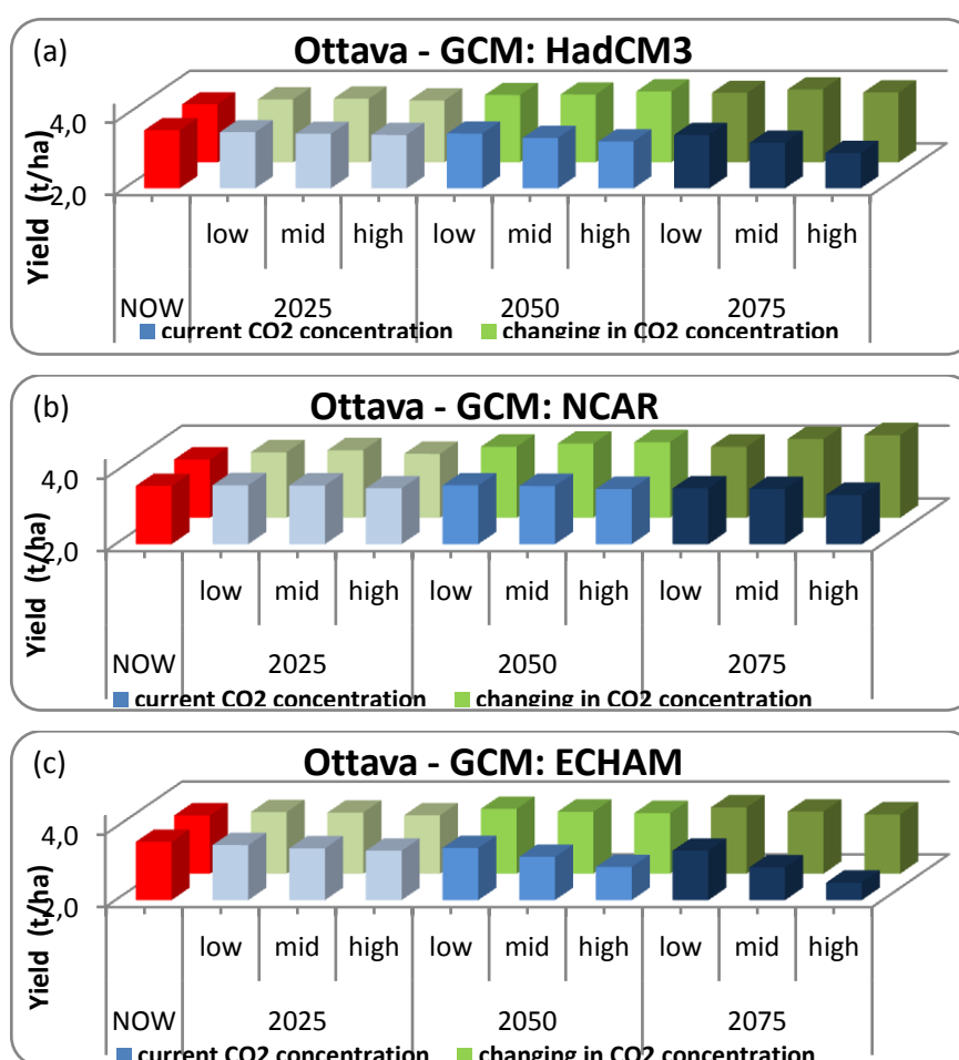
Fig. 4.3.1.1 a, b, c. Changes in yield ( \text{t ha}^{-1} ) from now to future periods, with current and future \text{CO}_2 concentration, with Hadley (a), NCAR (b) and ECHAM (c) GCMs and three climate scenarios (low, mid and high) for Simeto cultivar at Ottava site.
