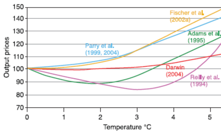
Figure 5. Cereal prices (percent of baseline) versus global mean temperature change for major modelling studies. Prices interpolated from point estimates of temperature effects (IPCC, 2007).
