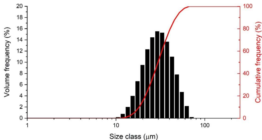
Figure 28. Particle size distribution of the CuNi 2 SiCr powder.
