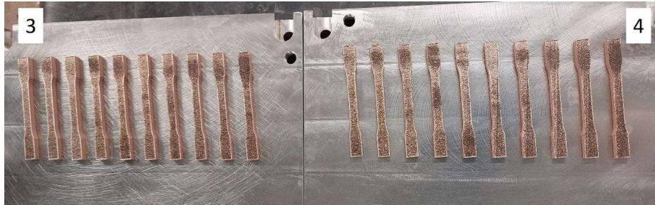
Figure 38. Printsharp CuNi 2 SiCr Batches 3 and 4 containing tensile samples.
