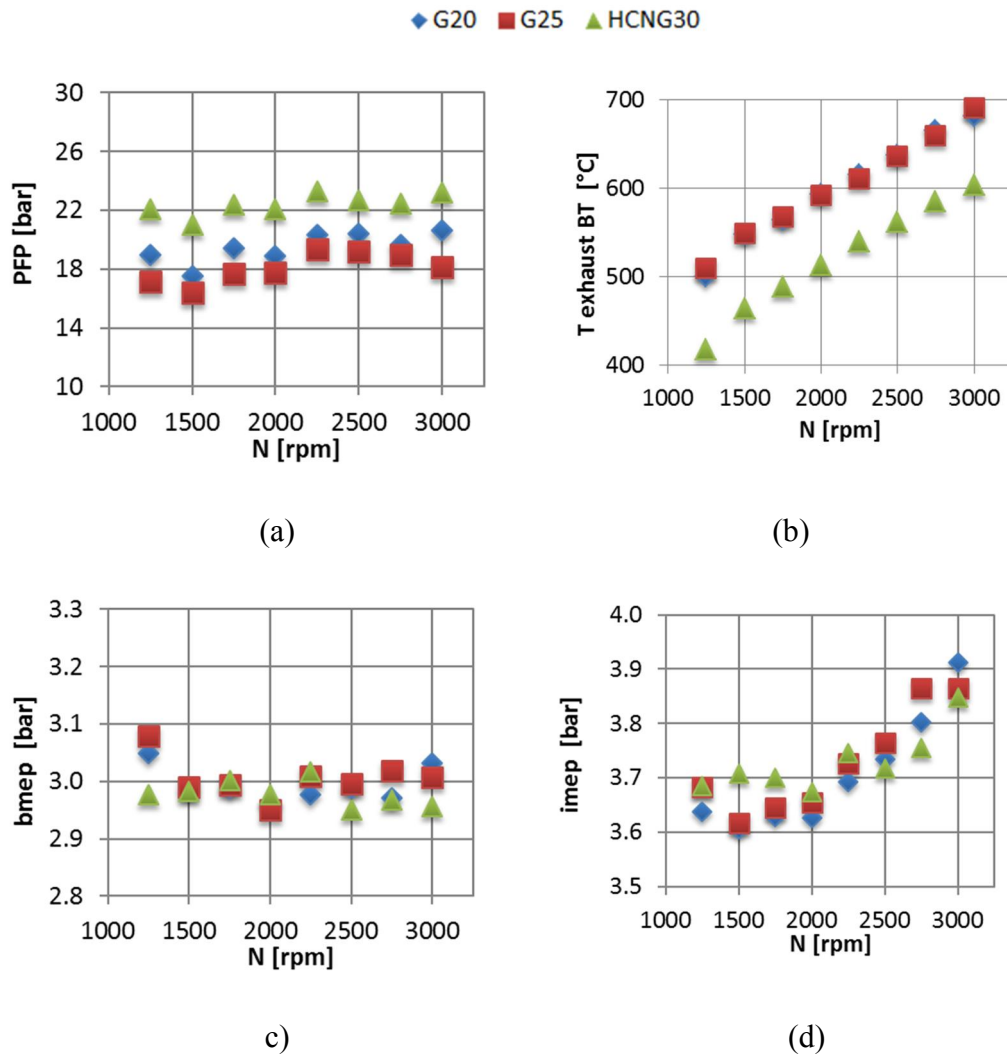
Figure 2.3 – Ensemble-averaged engine output over a speed sweep at nominal bmep=3bar .
