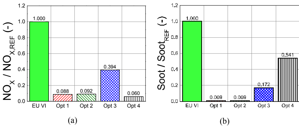
Figure 3.9 - NO x and soot brake specific emissions: comparison between the base EU VI calibration and the optimized PCCI points
