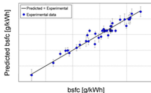
Figure 3.8 - bsfc: predicted vs. experimental values
