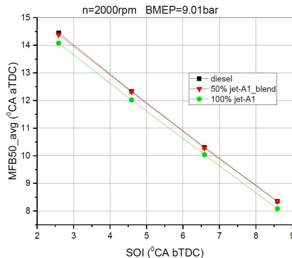
Figure 3.23 – Mean MFB50 versus SOI for the three tested fuels. Engine working point 2000×9.
