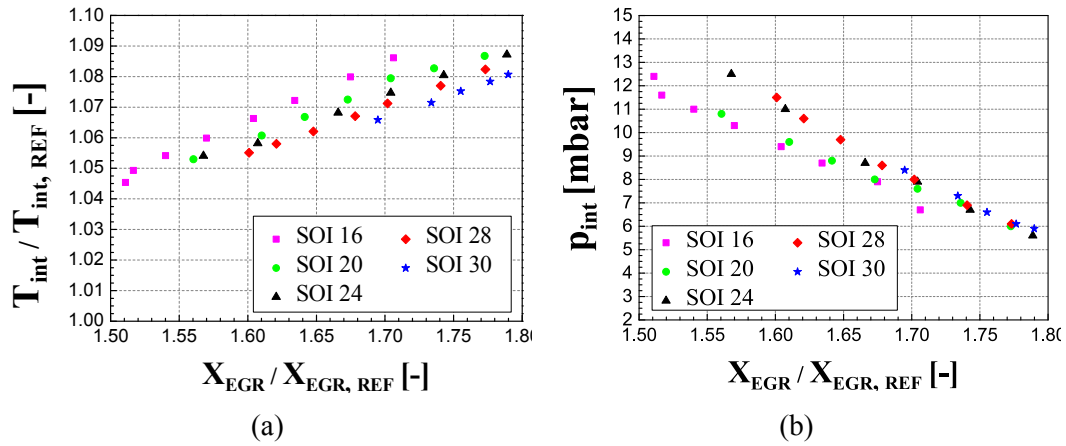
Figure 3.7 - (a) Intake manifold temperature vs EGR rate at different SOI; (b) Intake manifold pressure vs EGR rate at different SOI
