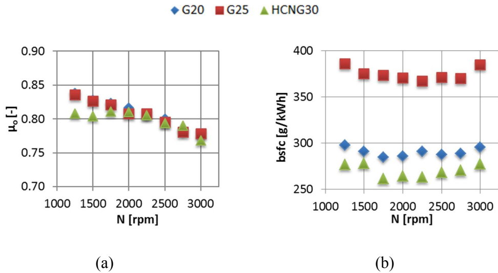
Figure 2.4 – Engine mechanical efficiency and brake specific fuel consumption at bmep=3bar.
