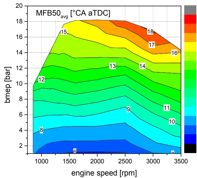
Figure 3.25 - Average MFB50 among cylinders as a function of engine speed and bmeep on engine mapping tests.
