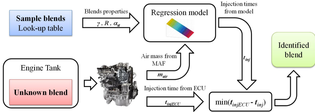
Figure 2.6 - Simplified flow-chart of the blend identification procedure.
