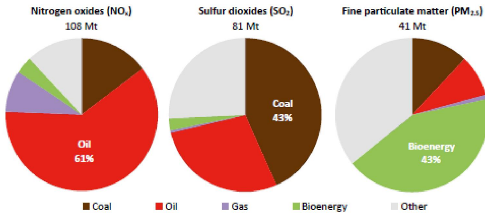
Figure 1.4 – Estimated anthropogenic emissions of the main air pollutants by source in 2015 according to World Energy Outlook 2016 (WEA 2016) proposed by the International Energy Agency (IEA).
