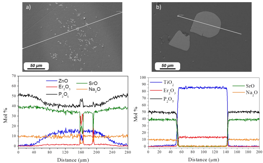
Figure 4.37 SEM pictures with their corresponding elemental mapping of Er 2 O 3 -doped ZnO (a) and TiO 2 (b) particles-containing glasses.
