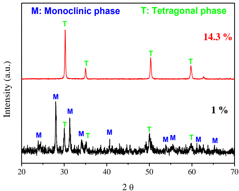
Figure 4.32 XRD patterns of 1 and 14.3 mol% \text{Er}_2\text{O}_3 -doped \text{ZrO}_2 particles calcined at 1000 °C for 2 h, with the reference pattern of the monoclinic and tetragonal crystalline phases.
