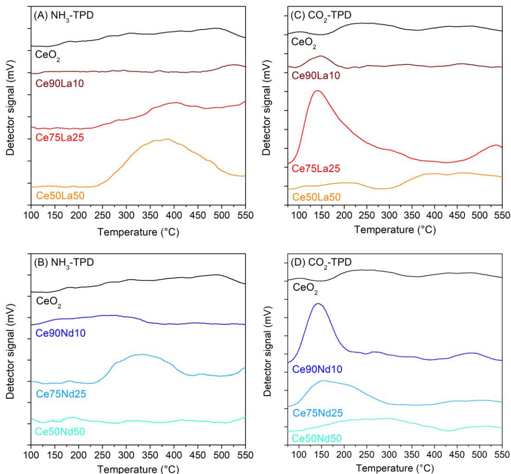
Figure 6.10. NH 3 -TPD (A, B) and CO 2 -TPD (C, D) profiles of the La-doped and Nd-doped samples compared with pure ceria.
