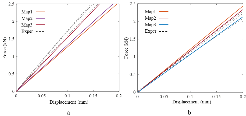
Figure 5.15. Experimental-numerical correlation of the specimen tested in tension: a) CP25 configuration; b) CP100 configuration.
