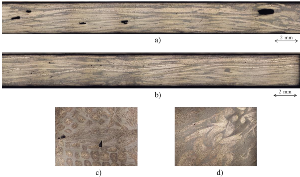
Figure 3.12. Micrographies of the CP100 and CP25 plates: a) cross-section of the CP100 plate; b) cross-section of the CP25 plate; c) surface detail of the chop interface region in the CP100 configuration; d) surface detail of the CP25 configuration.
