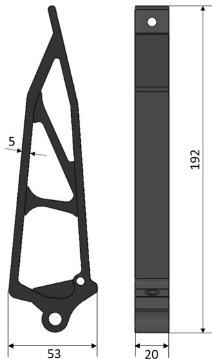
Figure 6.1. Pedal lever geometry. Dimensions are expressed in millimeters.
