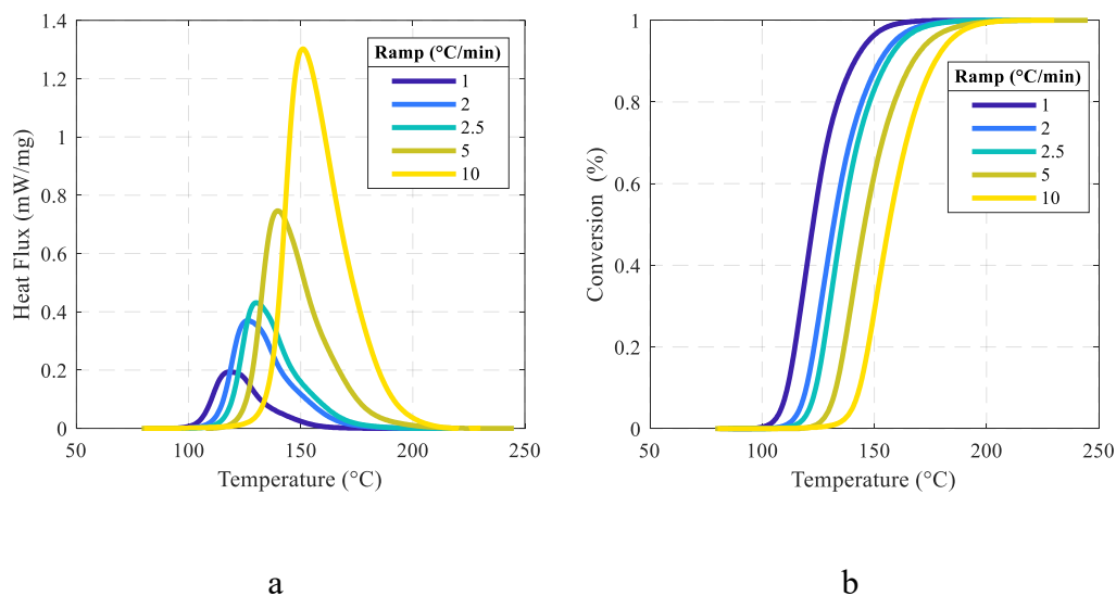
Figure 2.9. Dynamic DSC test results: a) Heat Flux vs Temperature; b) Conversion degree vs Temperature.
