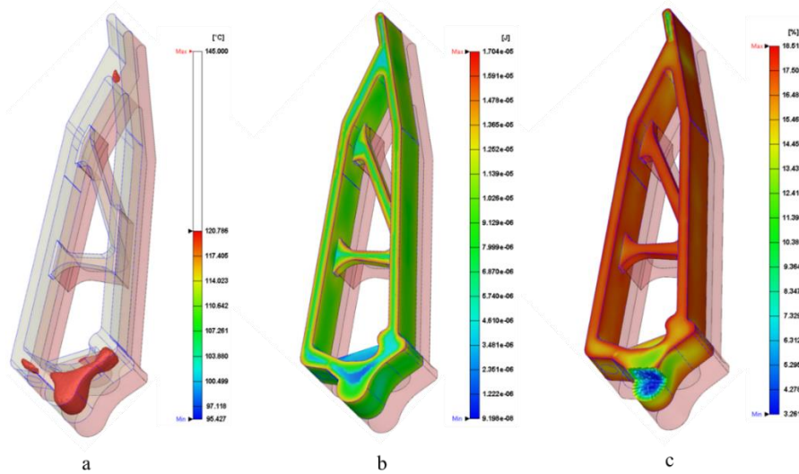
Figure 6.12. Simulation results: a) temperature of the material located in the hinge region; b) reactive heat generation; c) conversion state.
