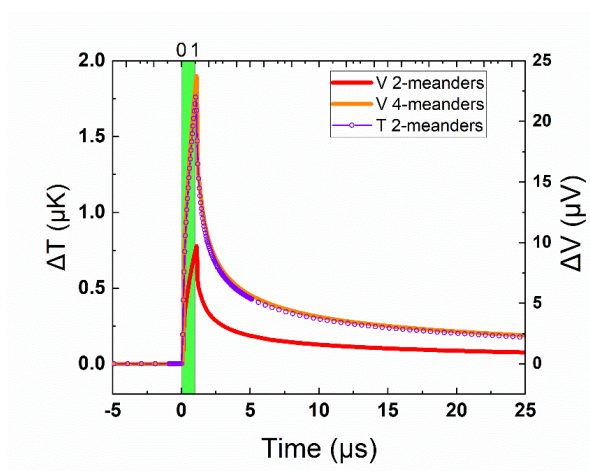
Figure 47: Response of the two bolometers, two and four meanders to a 1 \mu\text{s} signal
