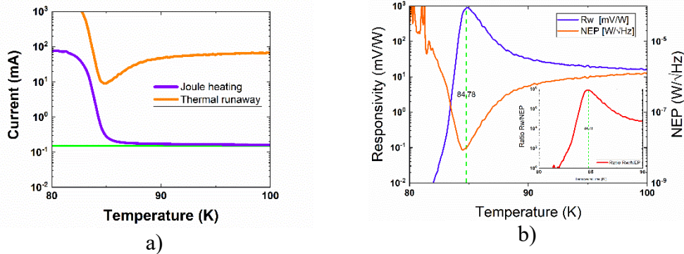
Figure 44: a) The study of bias current for the four-meanders configuration with the green line highlighting the chosen current, 0.15 mA and b) the study of the optimal working point with the responsivity (purple), the noise (orange) and their ratio (red)
