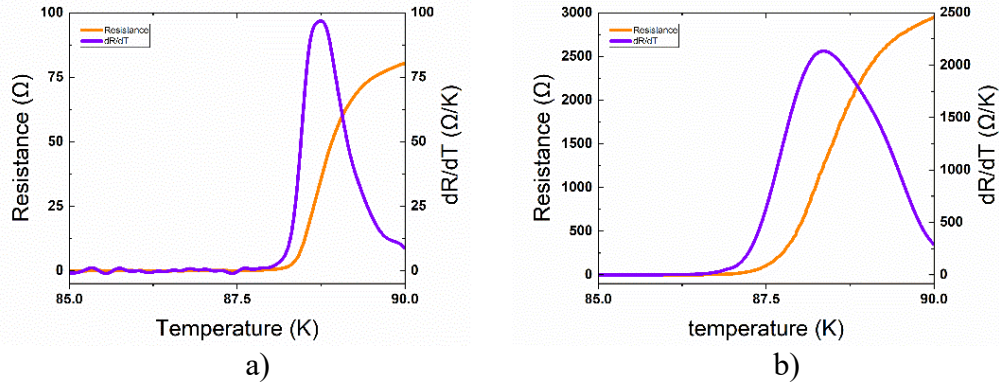
Figure 66: RvsT curve of the a) microbridge and b) the large serpentine
