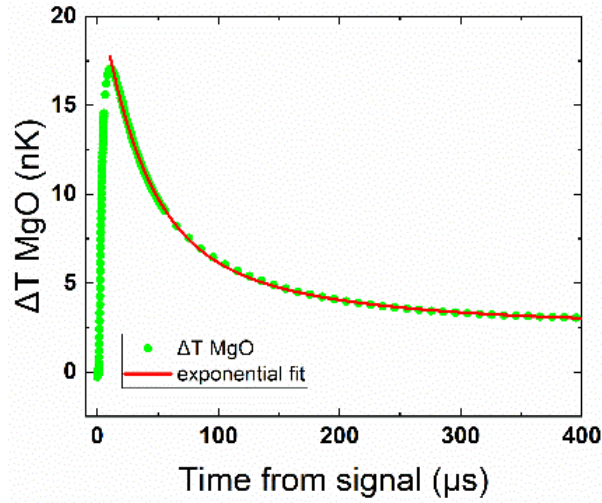
Figure 39: Temperature evolution at the center of the MgO substrate and its exponential fit
