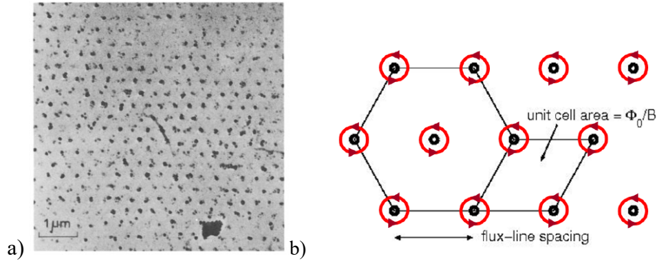
Figure 5: a) Distribution of the vortices in the superconductor. b) The sketch highlights the direction of the current and the geometrical distribution of the vortices
