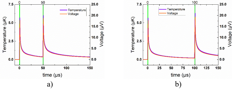
Figure 41: Response of the bolometer, the average temperature of the film and voltage drop, to two four pulses of length 1 \mu\text{s} and power 3 \text{ mW} separated by a) 50 \mu\text{s} and b) 100 \mu\text{s}
