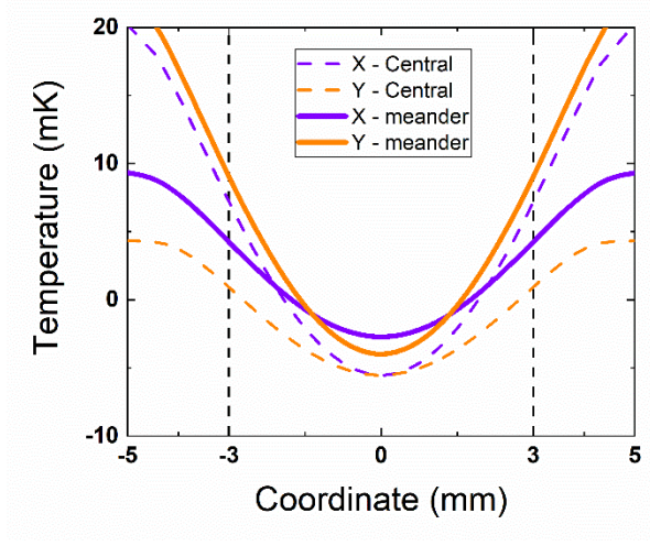
Figure 46: Linear profile for the line passing through the center of an irradiated meander (continue) and the center of the bolometer (dotted)
