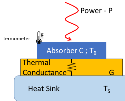
Figure 20: Main component of the bolometer
