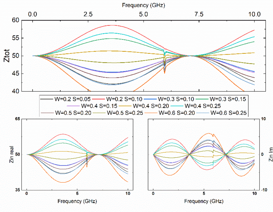
Figure 51: Input impedance for some configurations of the CPW optimization study
