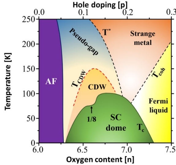
Figure 14: Phase diagram of \text{YBa}_2\text{Cu}_3\text{O}_{7-y} , as a function of hole doping p per planar copper atom and oxygen content n per unit cell
