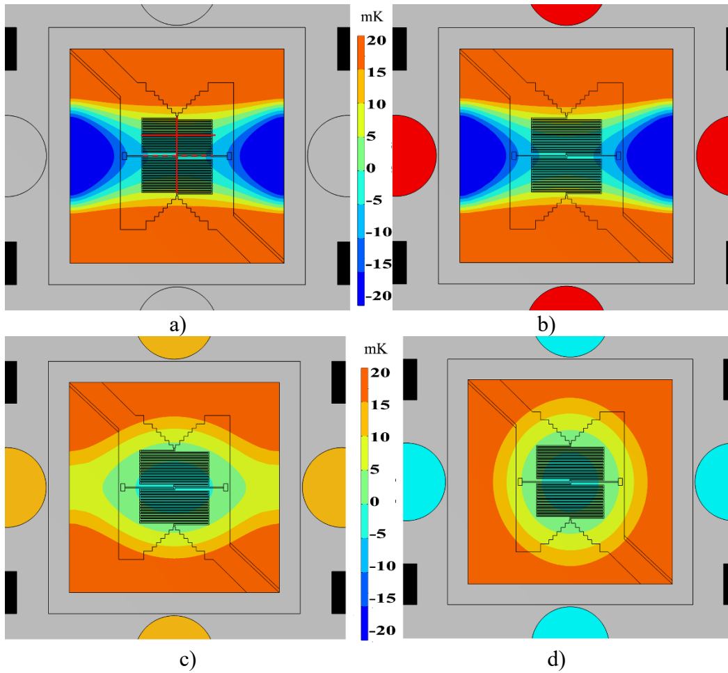
Figure 34: Differences from the working temperature (84.78 K) distribution for the various combination of screws on the aluminum (grey) holder: a) aluminum, b) copper, c) brass, d) Teflon ® . On a) the lines (red, straight and dashed) indicate where the linear profiles of the temperature are extrapolated
