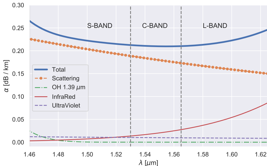
Fig. 2.2 A generic loss coefficient profile and the related model contributions.
