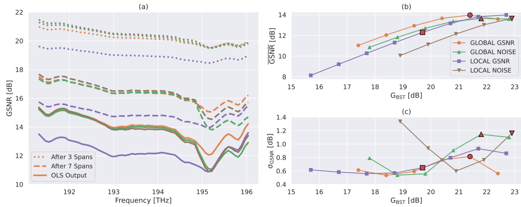
Fig. 3.20 Assessment on local vs. global optimization strategies: simulation results for the different optimization strategies: (a) GSNR profiles accumulated at different points of the OLS for the optimal configurations; GSNR aggregated metrics – (b) average, and (c) standard deviation – with respect to the BST gain varied in 1 dB steps (power sweep) at the end of the OLS.
