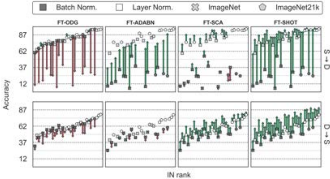
Figure 3.4 Example of fine-tuning impact for Modern Office31 dataset (Synthetic \rightarrow DSLR in the first row and DSLR \rightarrow Synthetic in the second row). Each marker is a backbone. Fine-tuning effect on the final accuracy is reported as arrows. In the first column, we report the accuracy variation between LP-ODG and FT-ODG (lower bound). Then, we report the accuracy difference with FT-ODG for the case when ADABN is applied (second column) and for FT-SCA and FT-SHOT (third and fourth columns).
