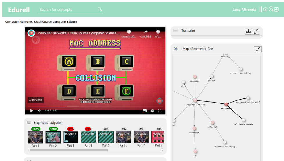
Figure 4.8: EVA interface
