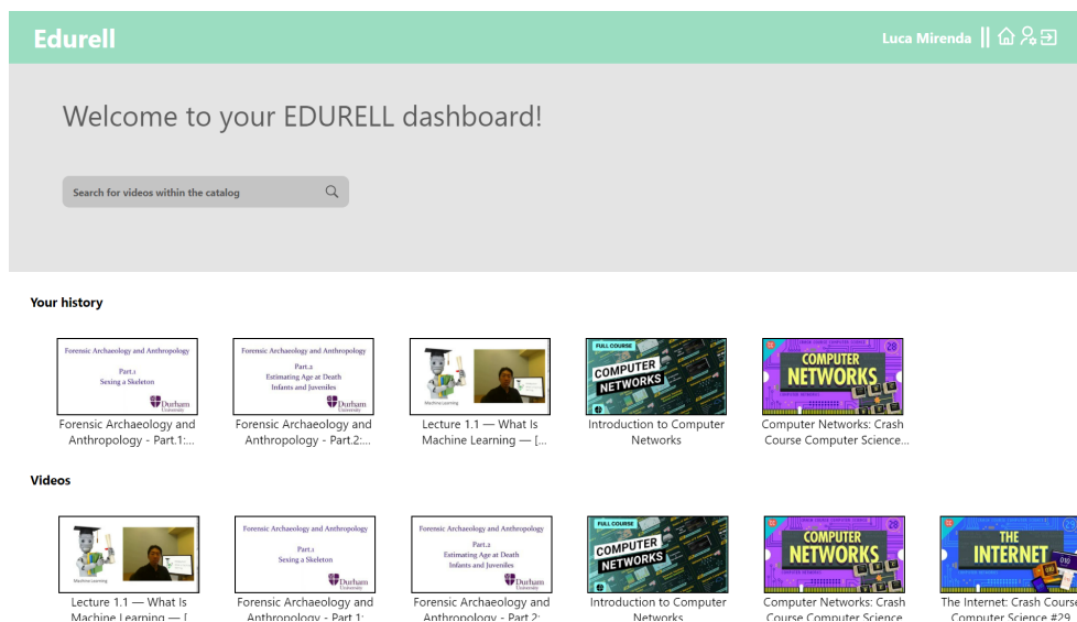
Figure 4.7: EVA dashboard
