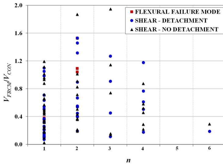
Figure 2-14 Variation of V_{FRCM}/V_{CON} with n
