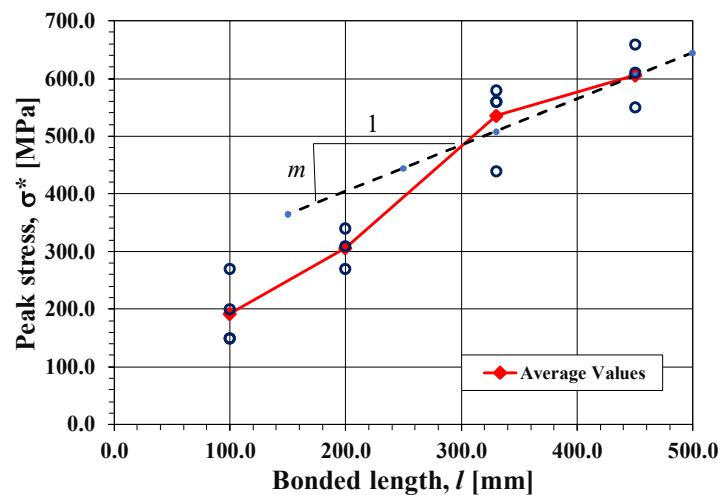
Figure 6-8 Peak stress \sigma^* vs. Bonded length l for carbon FRCM-concrete joints
