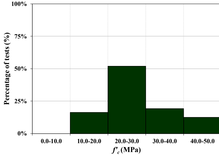
Figure 2-5. Data distribution for f'_c
