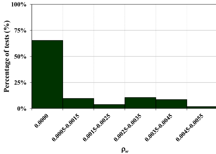
Figure 2-9. Data distribution for \rho_w
