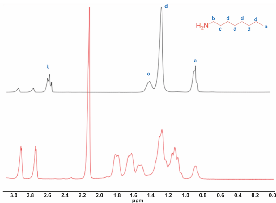
Figure 65. The 1 H-NMR spectrum of HCDs with internal standard (acetone) compared to that of octylamine.
