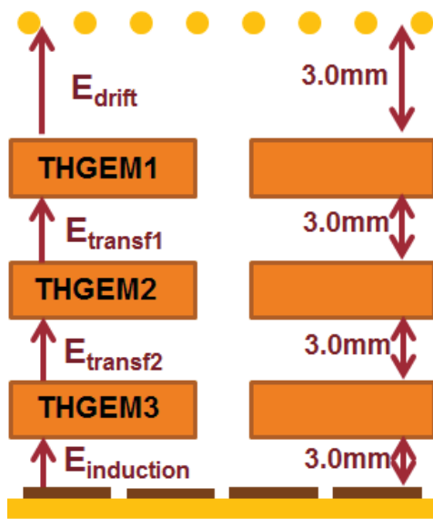
FIGURE 4.20: schematic of a multilayer THGEM setup.
