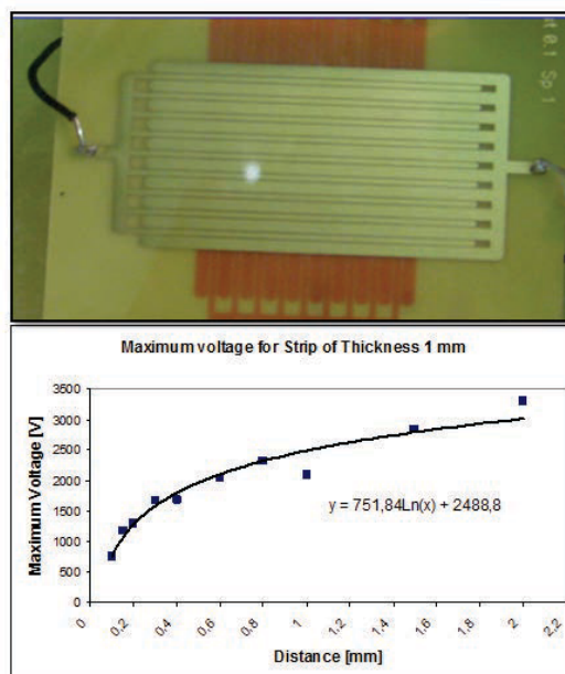
FIGURE 5.1: TOP: Picture of a discharge occurring during a study of the optimization of the THGEM segmentation performed with the special PCBs; BOTTOM: Measured breakdown voltage as function of the distance between electrode segments.
