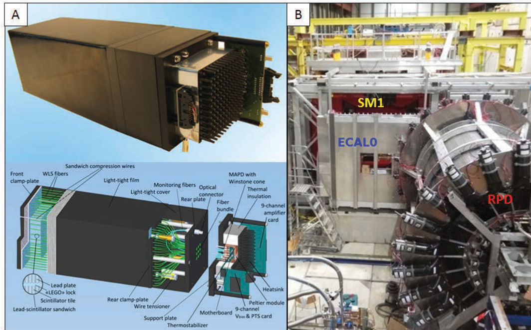
FIGURE 2.9: A. Top: a Shashlyk module with the MAPD connected to it. Bottom: Schematic of the Shashlyk module and MAPD system; B. View of COMPASS spectrometer setup inside the experimental hall 888 at CERN. Part of RPD detector, ECAL0 and the SM1 magnet (red color behind the frames) can be seen.
