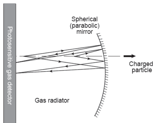
FIGURE 1.5: Schematic principle of a focusing RICH.
