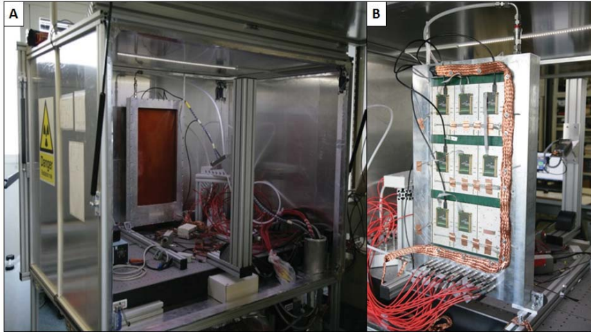
FIGURE 6.10: A. MINIX setup from the front. B. MINIX setup from back.
