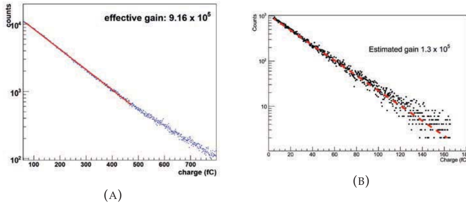
FIGURE 4.21: A. Single photo-electron amplitude spectra measured with the THGEM detector described in the text. B. Example of single photon amplitude spectrum from typical triple THGEM configurations; in particular, E_{TR1} = 2 kV/cm and E_{TR2} = 4 kV/cm.
