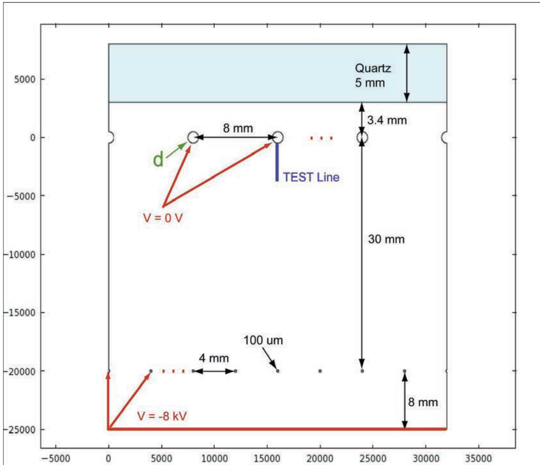
FIGURE 7.8: Schematic of COMPASS RICH-1 THGEM-based PD used for COMSOL field calculation
