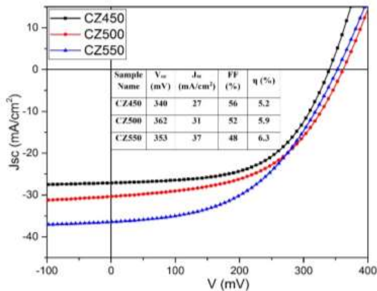
Figure 65. JV characteristics of CZTSSe devices fabricated.
