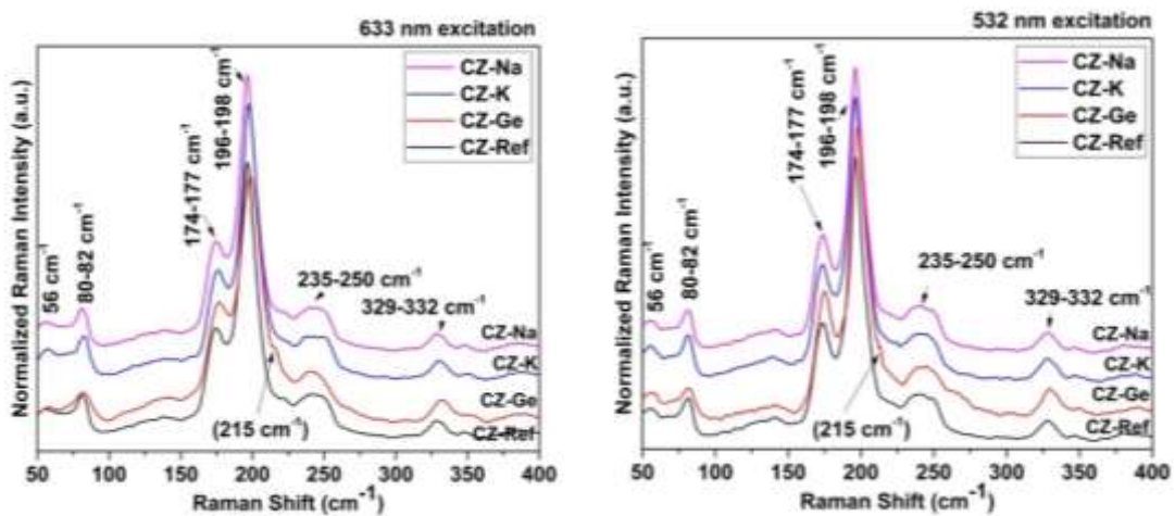
Figure 67. Raman spectra of untreated and treated materials excited by lasers at 633 nm and 532 nm: these spectra confirm for the treated absorbers a shift of the CZTSSe peaks with a larger shift for CZ-Ge and a smaller shift for CZ-Na (see figures 68 and 69).
