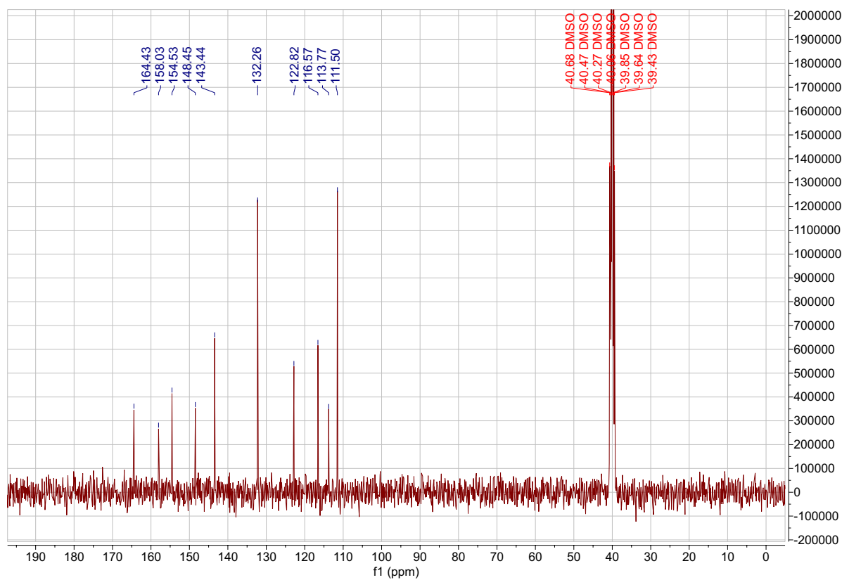
Supplementary Figure S17: ^{13}\text{C} NMR compound 45h (DMSO- d_6 ).
