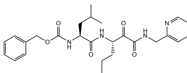
calpain inhibitor XII IC_{50} = 0.45 \mu\text{M}
