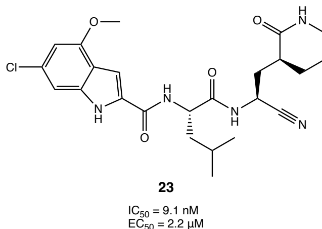
Figure 42. Chemical structure of the nitrile derivative 23 [180].
