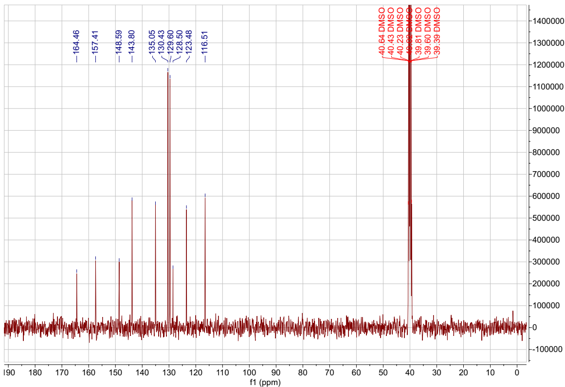
Supplementary Figure S15: 13 C NMR compound 45g (DMSO-d 6 ).
