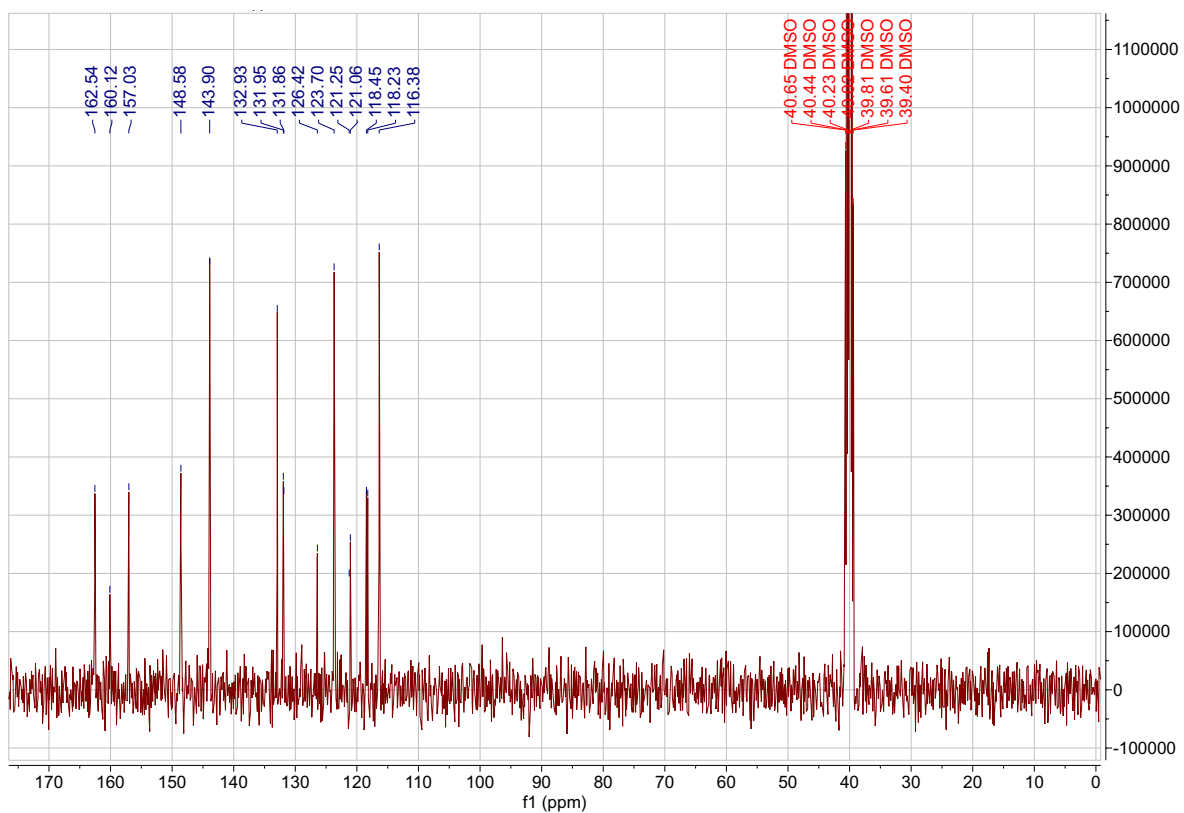
Supplementary Figure S27: 13 C NMR compound 45m (DMSO-d 6 ).
