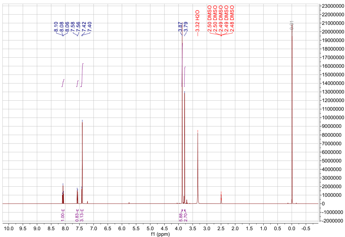
Supplementary Figure S6: 1 H NMR compound 45c (DMSO-d 6 ).
