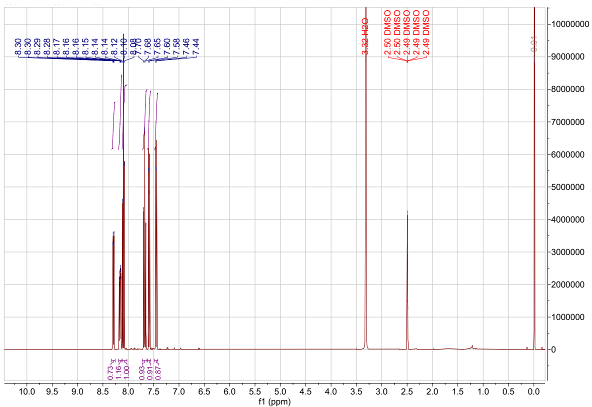
Supplementary Figure S26: 1 H NMR compound 45m (DMSO-d 6 ).
