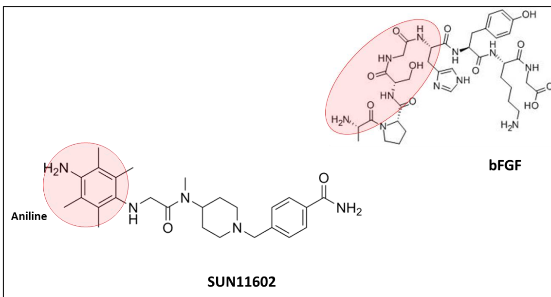
Figure 12. Structure of SUN11602, aniline derivate and mimetic of bFGF.
