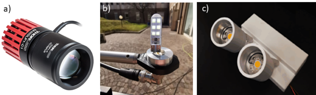
Figure 2.4: Images of main light sources used in experiments: a) 405 nm collimated light sources; b) automotive WLED; c) museum spotlight.
