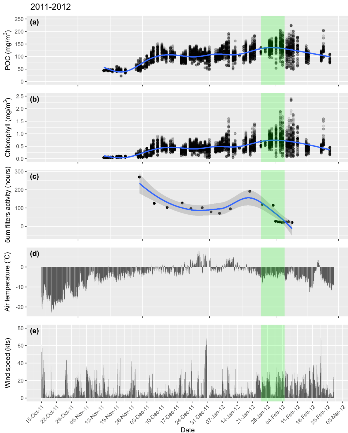
Appendix Figure 1: Daily satellite recordings of (a) Particulate Organic Carbon (POC) and (b) Chlorophyll, measured in milligrams per cubic meter. (c) 5 \mu\text{m} cartridge filters activity time measured in hours. Hourly recordings of AWS “Eneide” on (d) surface temperature and (e) wind speed for the MZS opening season 2011-2012. Blue lines are the smoothing lines, with the grey areas depicting the confidence intervals around the smoothing, according to a generalized additive model for (a) and (b), and to a loess approximation for (c). Green shaded areas highlight the investigated time range, from the installation day of the first filter to the sampling day of the last one.
