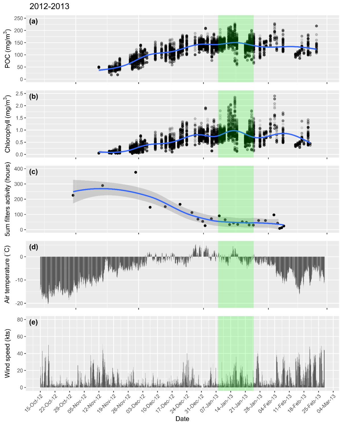
Appendix Figure 2: Daily satellite recordings of (a) Particulate Organic Carbon (POC) and (b) Chlorophyll, measured in milligrams per cubic meter. (c) 5 \mu\text{m} cartridge filters activity time measured in hours. Hourly recordings of AWS “Eneide” on (d) surface temperature and (e) wind speed for the MZS opening season 2012-2013. Blue lines are the smoothing lines, with the grey areas depicting the confidence intervals around the smoothing, according to a generalized additive model for (a) and (b), and to a loess approximation for (c). Green shaded areas highlight the investigated time range, from the installation day of the first filter to the sampling day of the last one.
