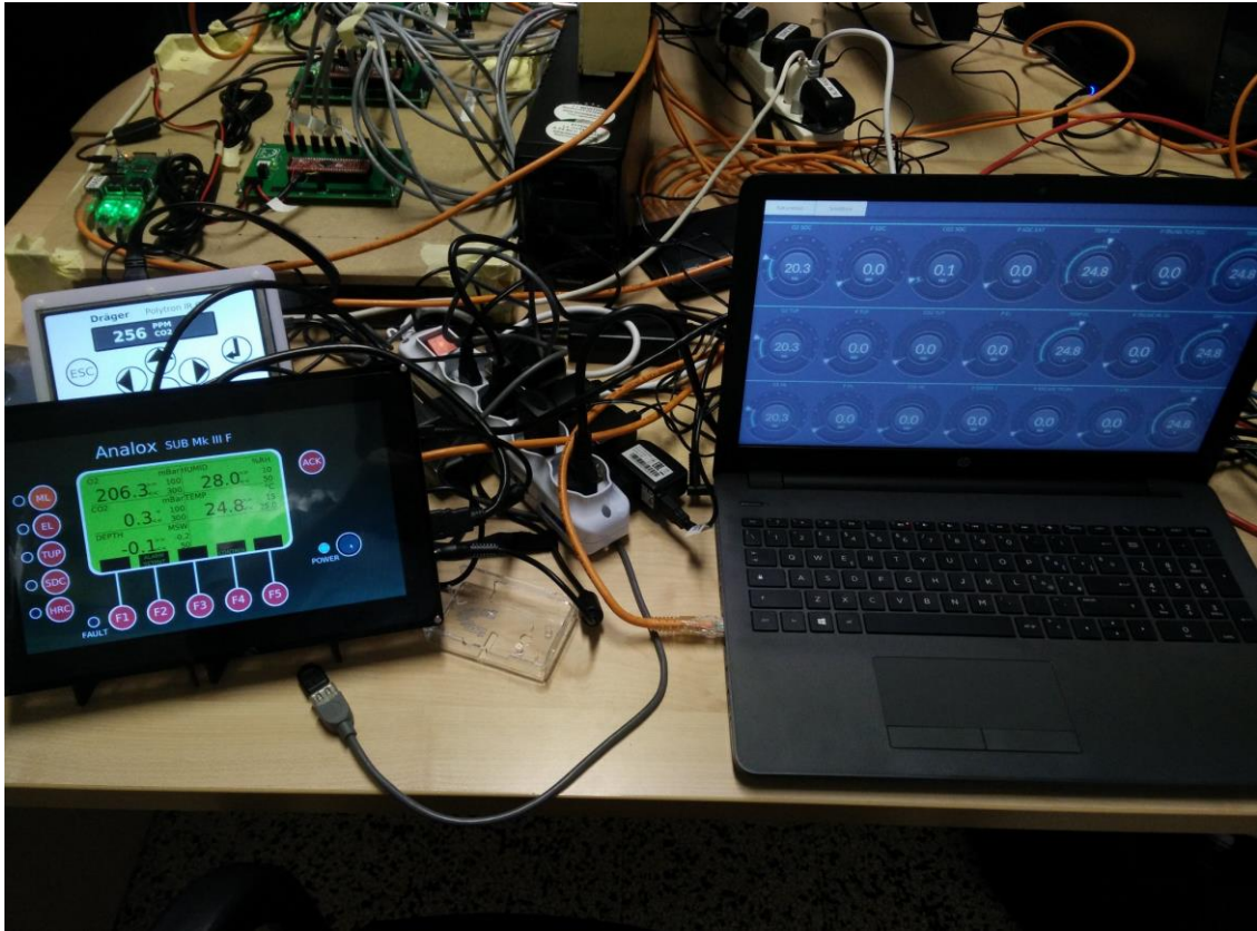
Figure 7-9. First integration test combining prototypes of 3 atmospheric monitoring systems and analysers and mock-up of valves and pressure gauges
