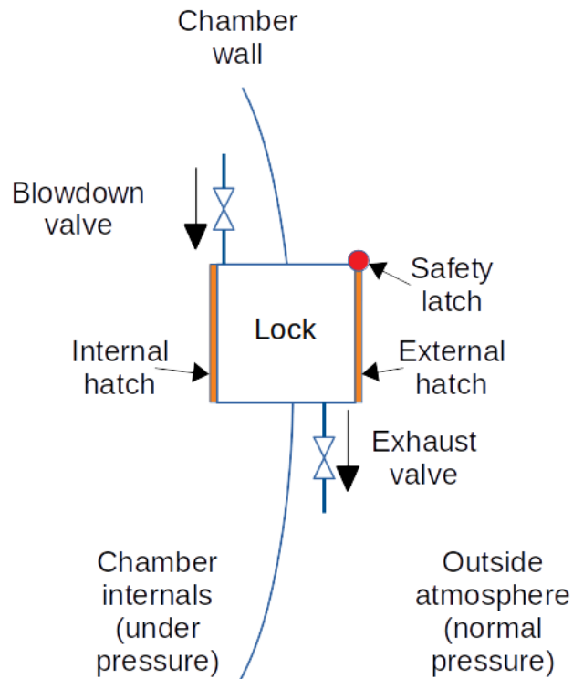
Figure 2-4. Material and food passing locks' structure.
