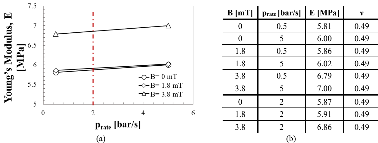
Figure 5.13 (a) Trend of Young's Modulus, E according to pressure rate, p_{rate} resulting from the inverse analysis procedure; (b) summary of values of E and \nu after the the inverse analysis procedure for p_{rate}=0.5 bar/s and p_{rate}=5 bar/s; E and \nu prediction for p_{rate}=2 bar/s.
