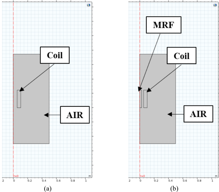
Figure 3.21 Comsol FE model for the evaluation of the magnetic flux density
