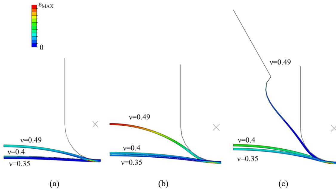
Figure 5.12 Major strain map for p_{rate}= 0.5 bar/s and different values of v when (a) E=1 MPa (b) E= 5 MPa and (c) E= 15 MPa
