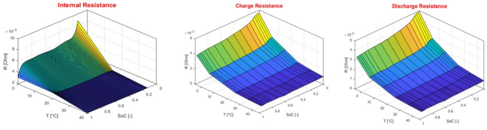
Figure 73: HV battery cell internal resistance for LiPo (left) and Li-NMC in charge (center) and discharge (right)
