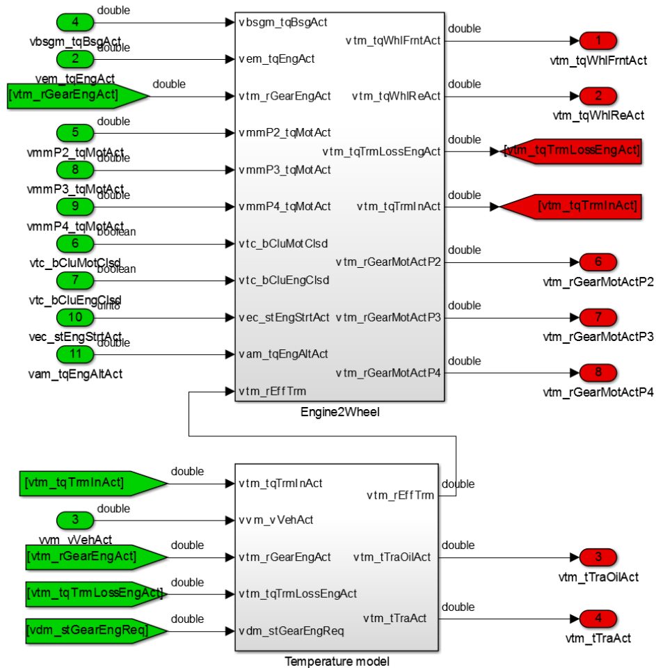
Figure 65: Physical transmission model
