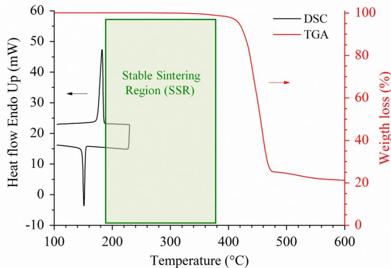
Figure 63: Graphical representation of the stable sintering region for PA12/CF powders. DSC thermogram (left axis) and TGA curve in air atmosphere (right axis) are reported in the graph
