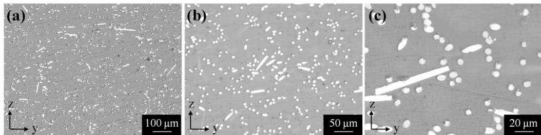
Figure 70: Optical micrographs of YZ cross section of PA12/CF parts sintered with energy density of 0.233 \text{ J/mm}^3 : (a) low magnification image, (b) detailed view of the distribution of carbon fibers in the polymer matrix and (c) high magnification image showing the fiber/matrix interfaces
