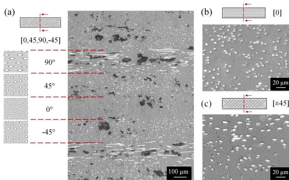
Figure 85: Optical micrographs of the polished YZ cross sections of PA6/CF samples printed with various architectures: (a) [0/45/90/-45], (b) [0] and (c) [ \pm 45]. In figure (a) the cross sectional shapes of the fibers observed in the stacked layers are schematically sketched
