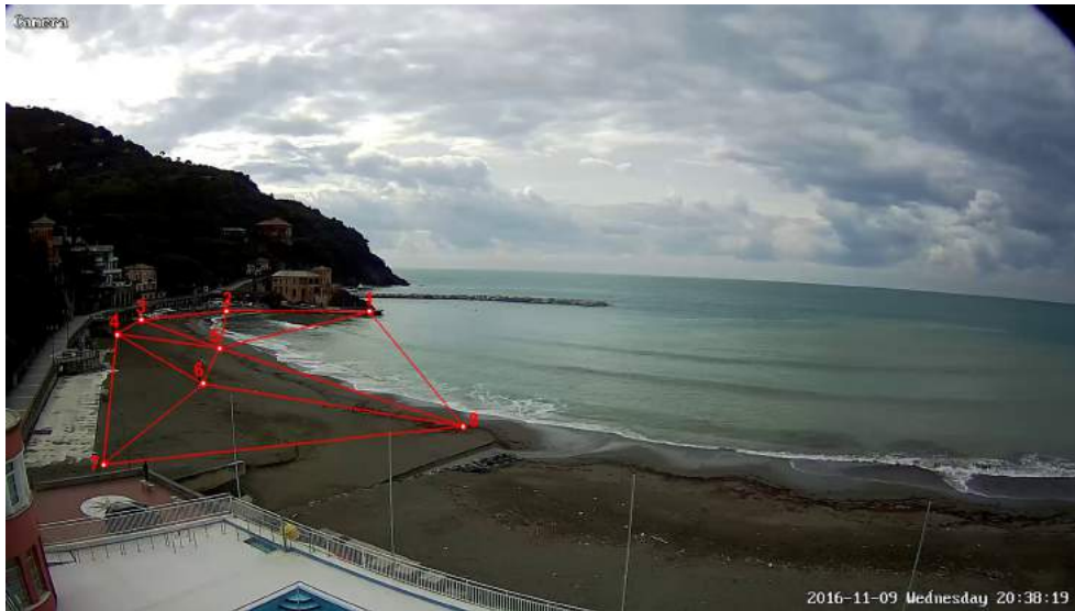
Figure 4.6: Example of Ground Control Points (GCPs) triangulation along the eastern sector of the beach.
