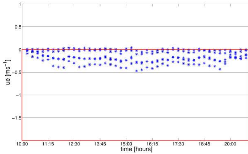
Figure 5.19: Rip current behaviour on the west side of the groyne, rip generation sector 2 (S.2).
