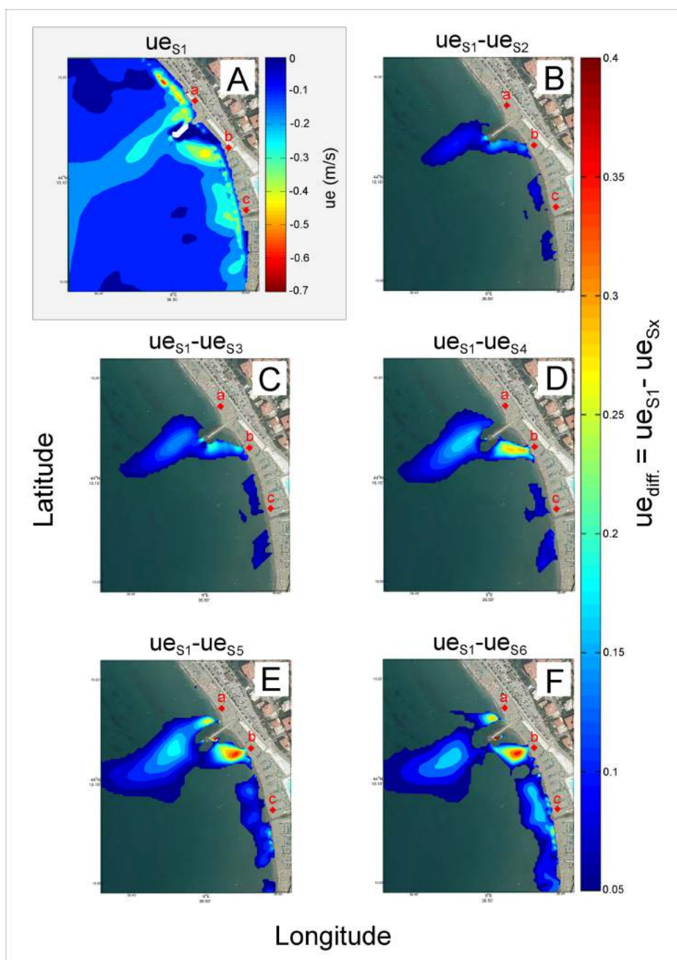
Figure 5.46: Panel A. Average values of ue in scenario 1 ( S1 ). panels B, C, D, E, F. Difference between ue magnitude in scenario 1 ( S1 ) and ue magnitude under sea-level change scenarios ( S2 , S3 , S4 , S5 , S6 ).
