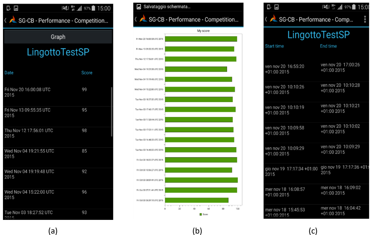
Figure 26: (a) User scores in each competition (b) Graphical representation of scores (c) list of competition instances.
