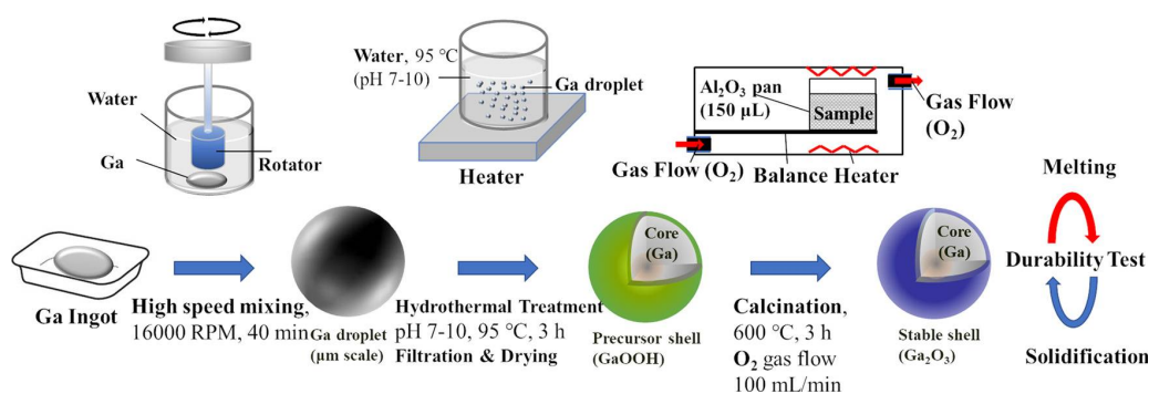
Figure 4.3: Schematic diagram of the \text{Ga}_2\text{O}_3 MEPCM fabrication process. The figure is taken from [160].
