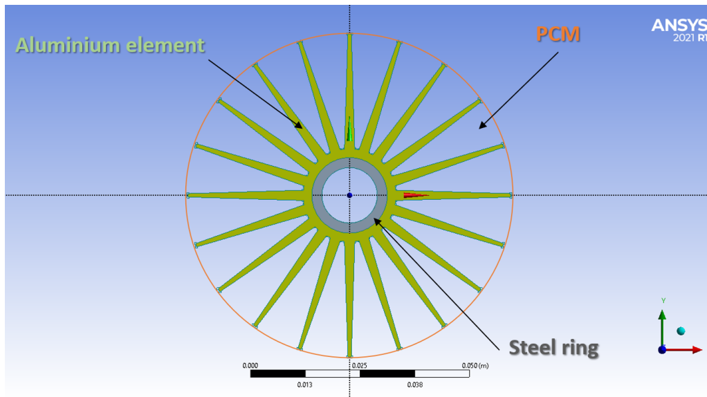
Figure 4.18: One of the three different geometries studied in the present work. It has a steel inner tube for Heat Transfer Fluid flow (grey element) and an aluminum heat conduction structure connected to the heat transfer tube (green component). The PCM is all around the aluminum structure up to its outer radius.
