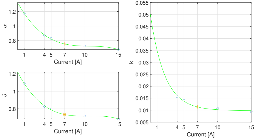
Figure 2.26: Free parameter plots with p = 65 \text{ rad/s} - \alpha and z = 100 \text{ rad/s}^{1-\beta} , the corresponding interpolation laws (in green) and the fitted working point at 7 A (in red).
