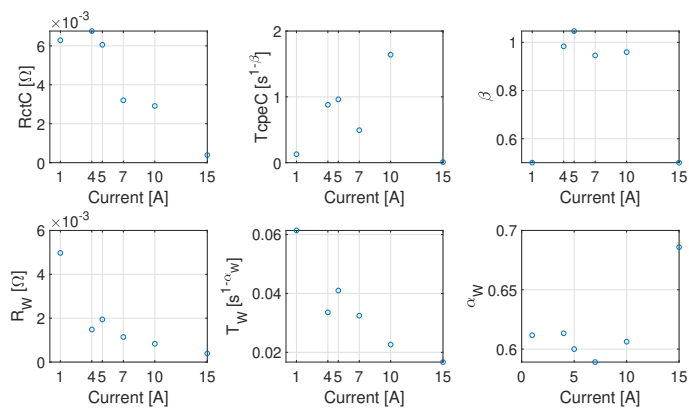
(b) High-current Dhirde et al. EECM parameters: R_{ct,C} , T_{cpe,C} , \beta , R_W , T_W , and \alpha_W .
