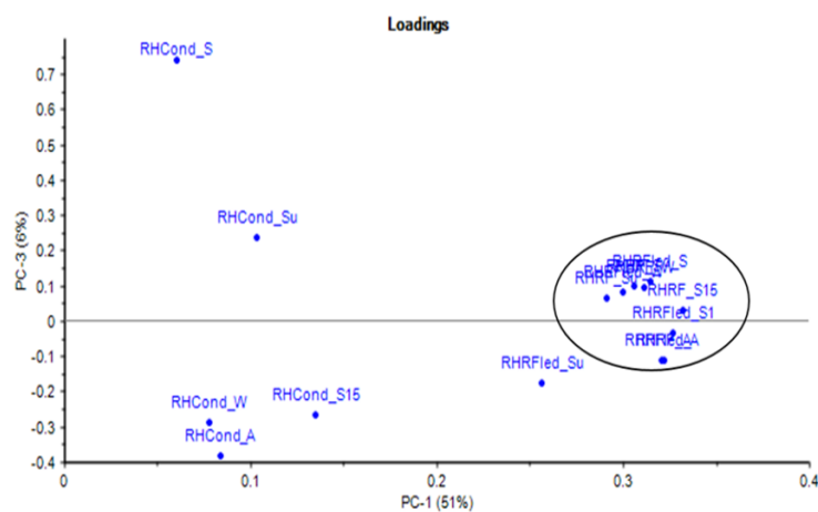
Figure 3. PC3 Loadings.
