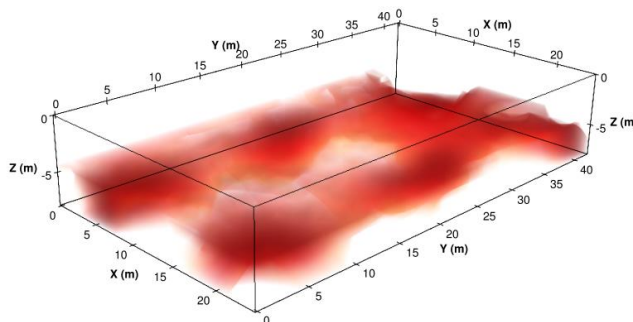
Figure 7. Volumetric image of the "Casa di Diana" foundation walls, obtained mapping only elements deeper than 4 m with resistivity values higher than 50 \Omega\text{m} . Image made using Kitware Paraview.
