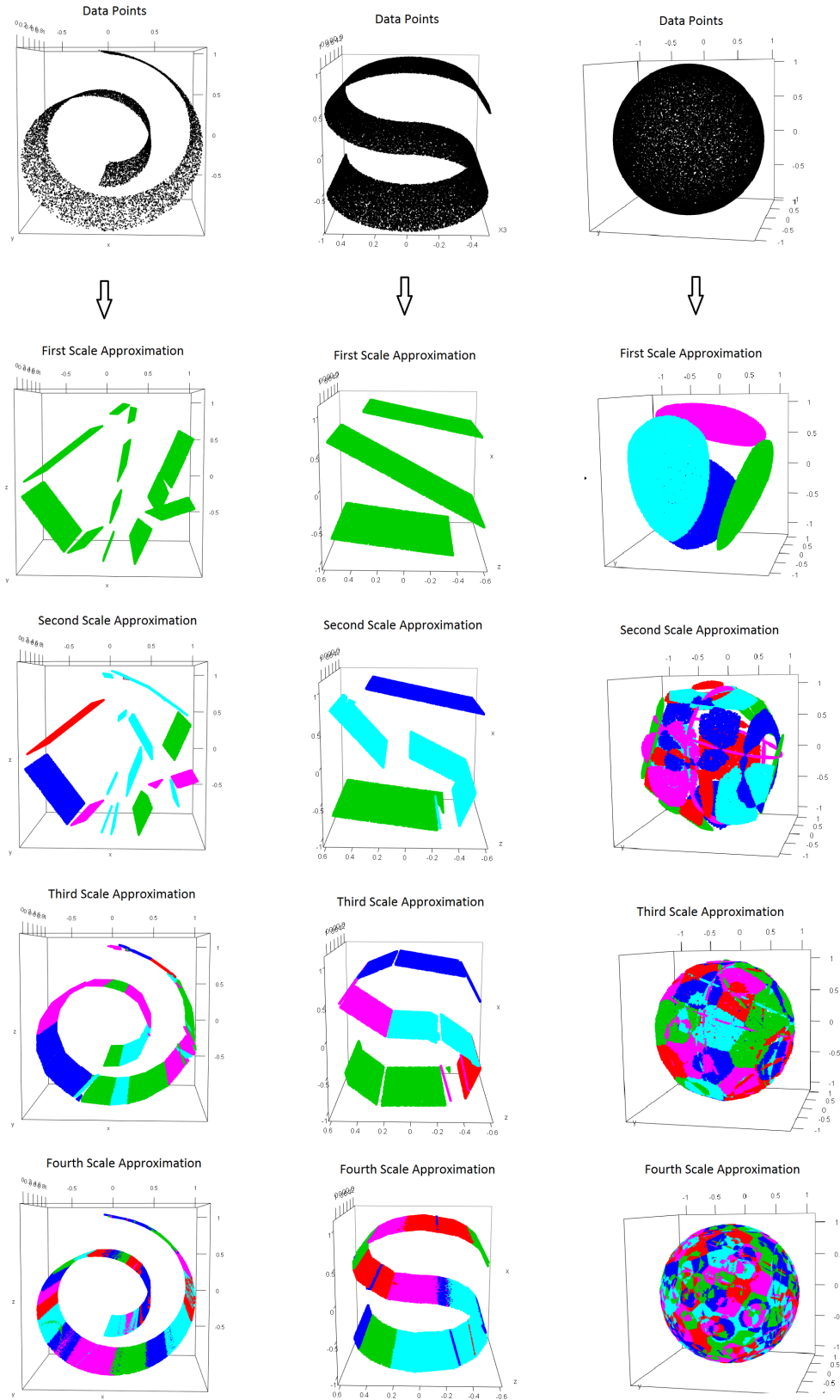
Figure 6.3: An example of the multiscale reconstruction on three different manifolds: a Swissroll, a S-Shaped manifold and a surface of a 3D sphere. All these manifold are embedded in \mathbb{R}^{30} and then corrupted with gaussian noise.
