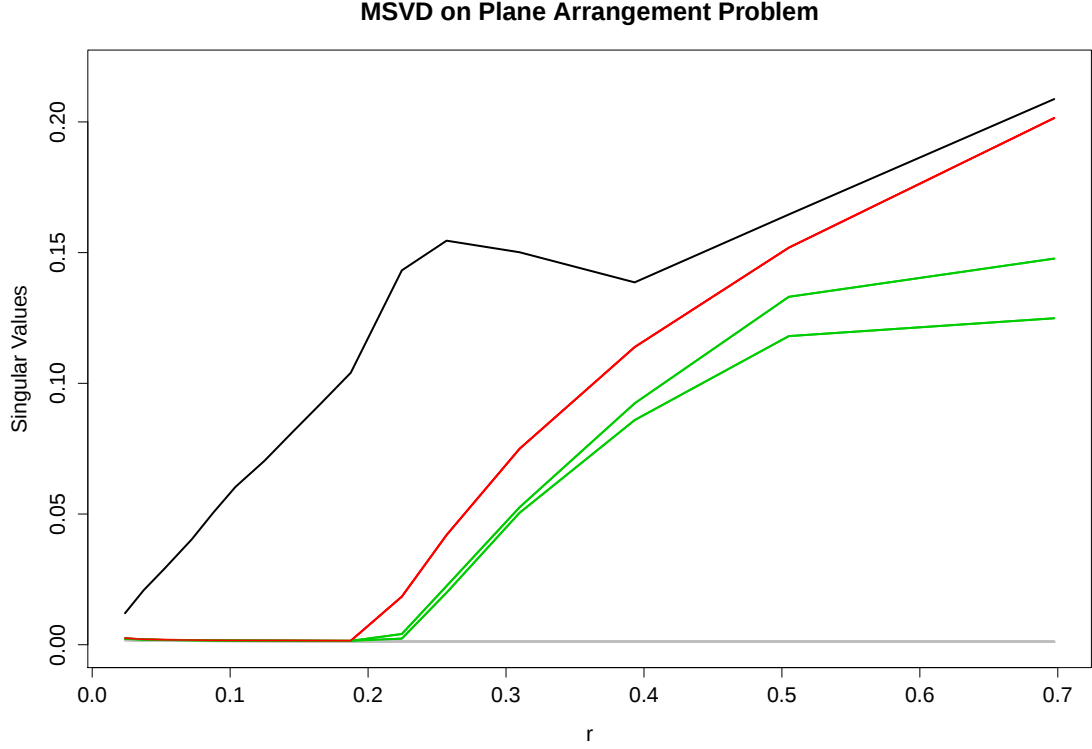
Figure 5.2: A Representative image of a MSVD on the data shown in Figure 5.1. We use for center x a point generated from the black plane ( d = 1 ). Here one can appreciate the behavior described in Section 5.2. For small values of r only the first SV grows almost linearly. As r increase, around 0.2, the neighborhood of x includes points of the red plane ( d = 1 ) and the second SV starts to grow linearly too. Around r = 0.23 the sphere hits the green plane ( d = 2 ), thus, the next two SVs start to grow linearly. The remaining 2 = (D - \sum_{k=1}^K d_k) SVs stay flat because they represent only noise. Note: in typical applications we do not know a priori from which plane x is generated or in which order the planes are hit by the sphere, the colors of this figure are only chosen for the sake of a better comprehension.
